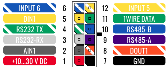
FMB125 2x6 socket pinout
