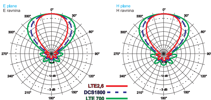
Radiation pattern Smerni diagram
